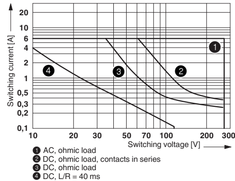
Interrupting rating
